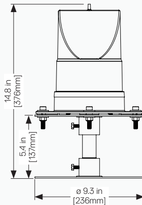
AV-70 WITH FRANGIBLE CONCRETE MOUNT (OTHER MOUNTING OPTIONS AVAILABLE)
