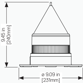
AV-70 WITH FRANGIBLE CONCRETE MOUNT (OTHER MOUNTING OPTIONS AVAILABLE)
